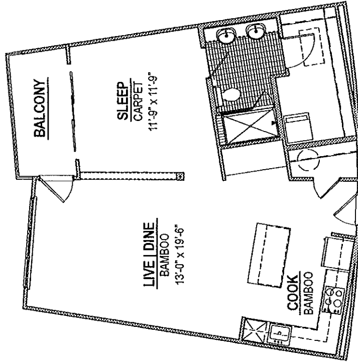
LEVEL 2 & 3 - 790 SQUARE FEET [HEATED SQUARE FOOTAGE]
